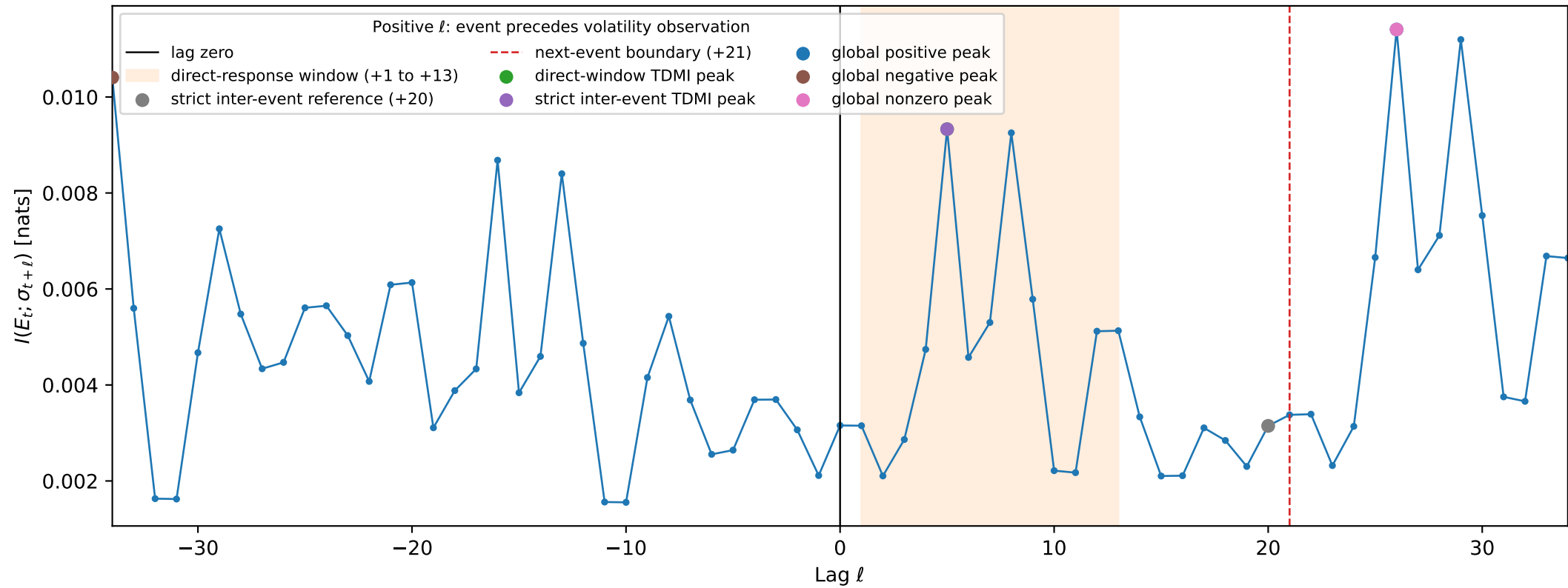
TDMI: E_t and \sigma_{t+\ell}
